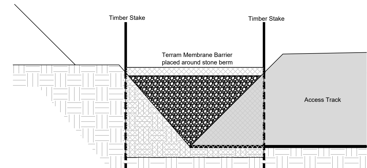
Sediment Fence Detail Scale 1:20
