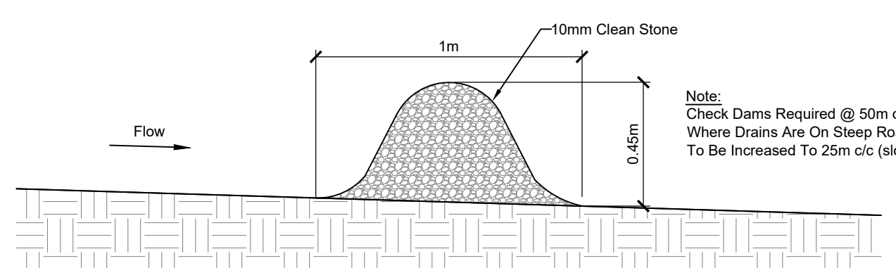
Check Dam Detail Scale 1:30
