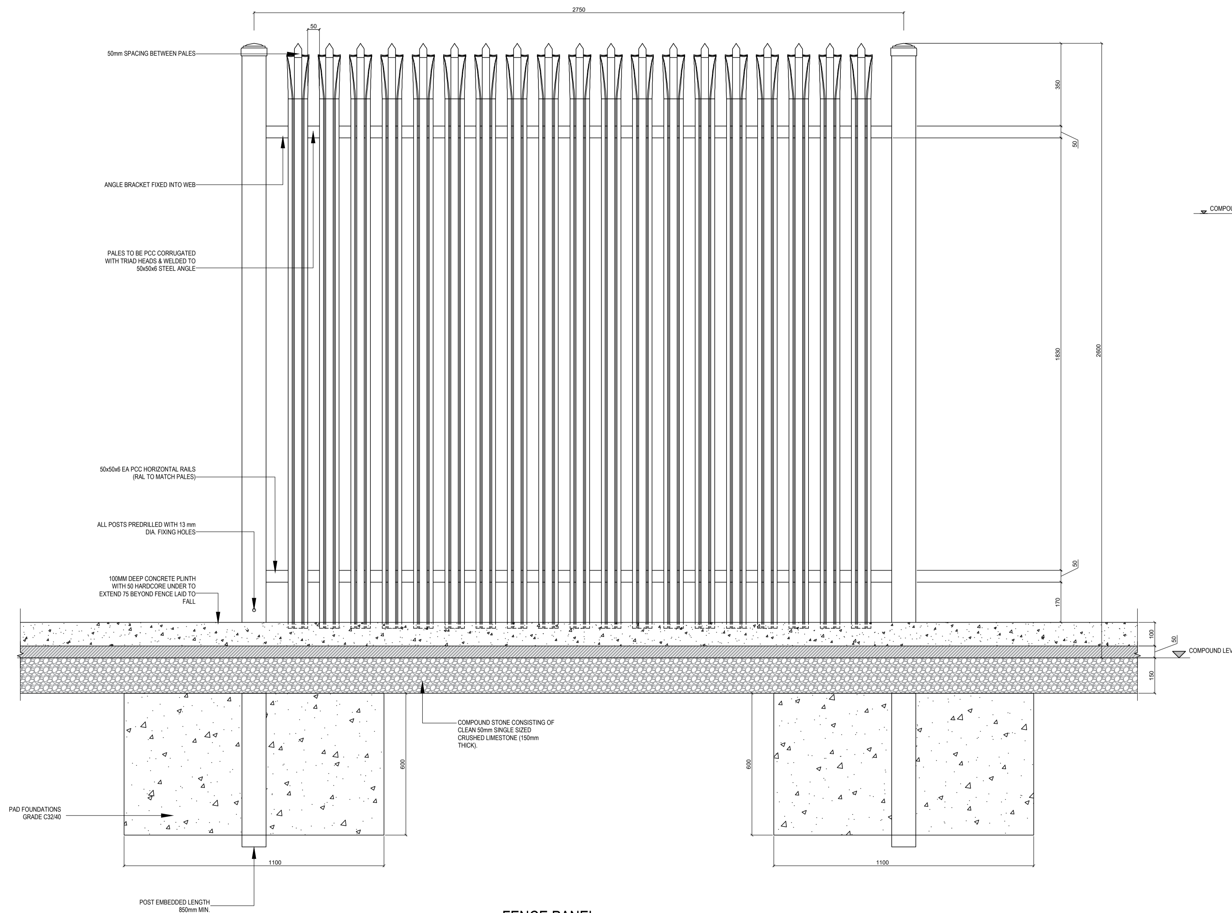
FENCE PANEL ELEVATION SCALE 1: 10
