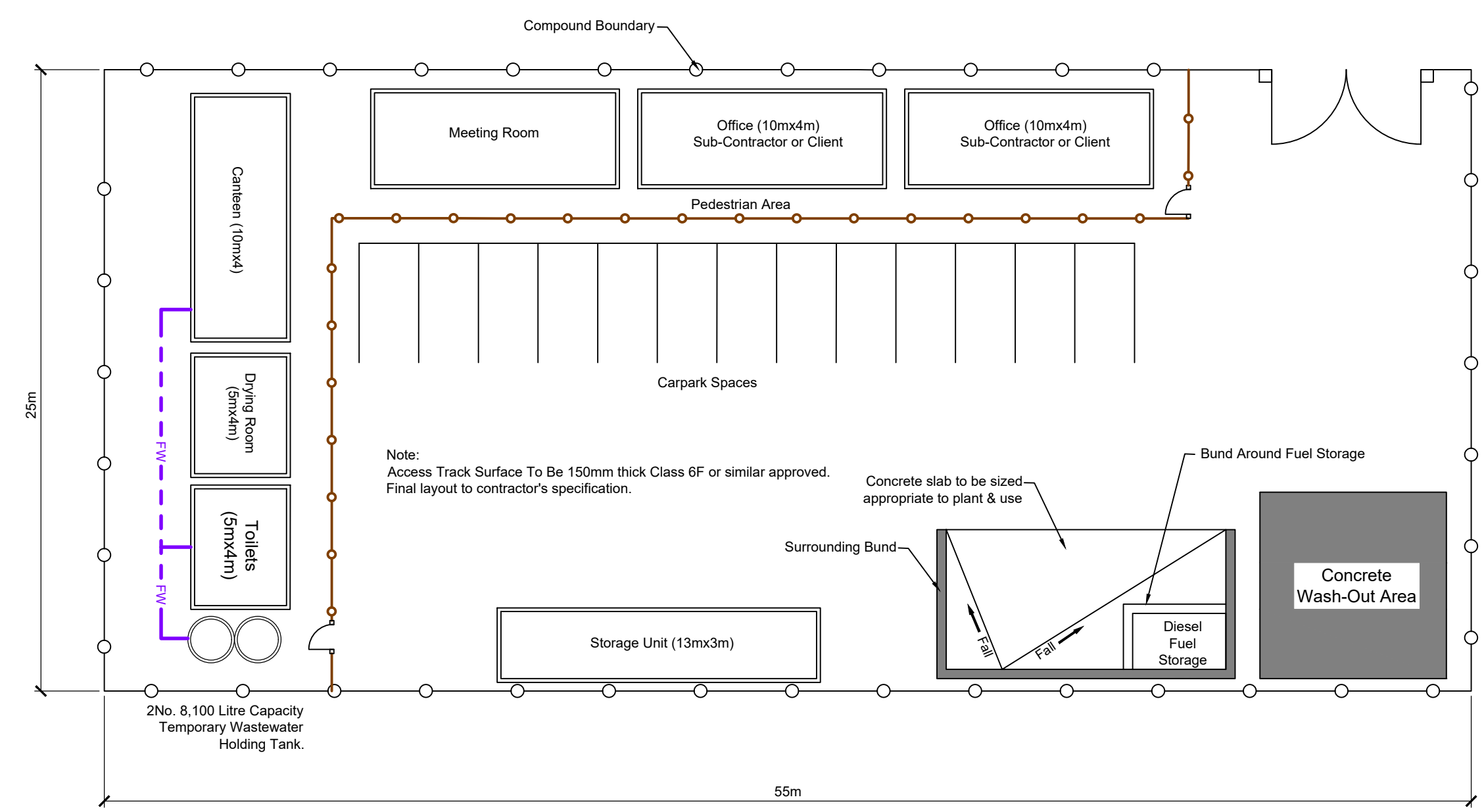
Temporary Site Construction Compound No. 2 Layout Scale 1:250
